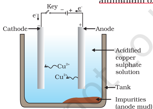
Figure 3.12 Electrolytic refining of copper. The electrolyte is a solution of acidified copper sulphate . The anode is impure copper, whereas, the cathode is a strip of pure copper. On passing electric current, pure copper is deposited on the cathode.
